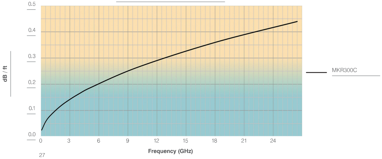
POWER HANDLING
