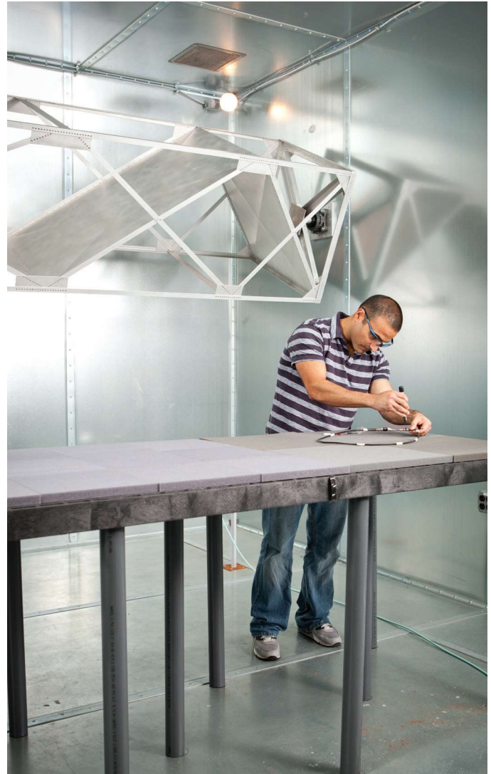
Mode stir RF-Shielding testing per IEC Standard 61000-4-21 Annex F
