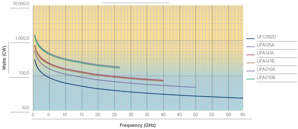
POWER HANDLING
